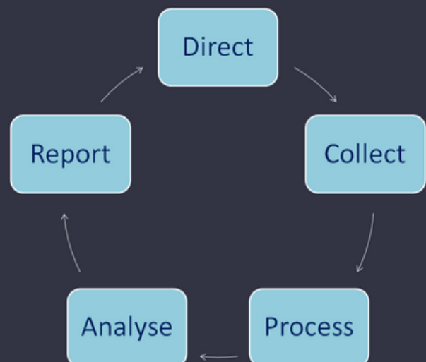
Figure 1: Intelligence Cycle
